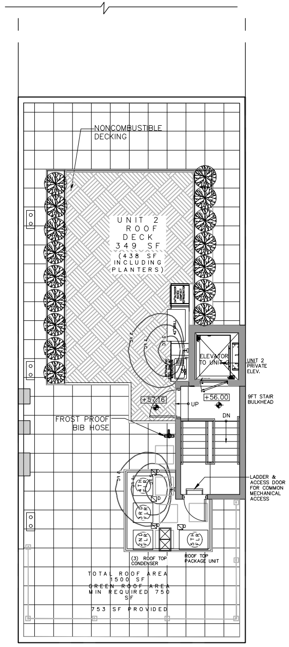
ROOF: UNIT 2 SCALE: 3/32"=1'-0"
