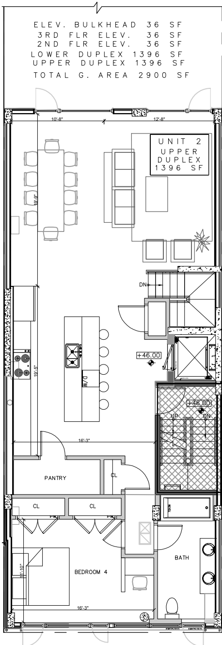
FIFTH FLOOR: UNIT 2 SCALE: 3/32"=1'-0"
