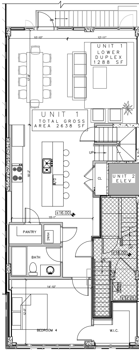
SECOND FLOOR: UNIT 1 SCALE: 3/32"=1'-0"
