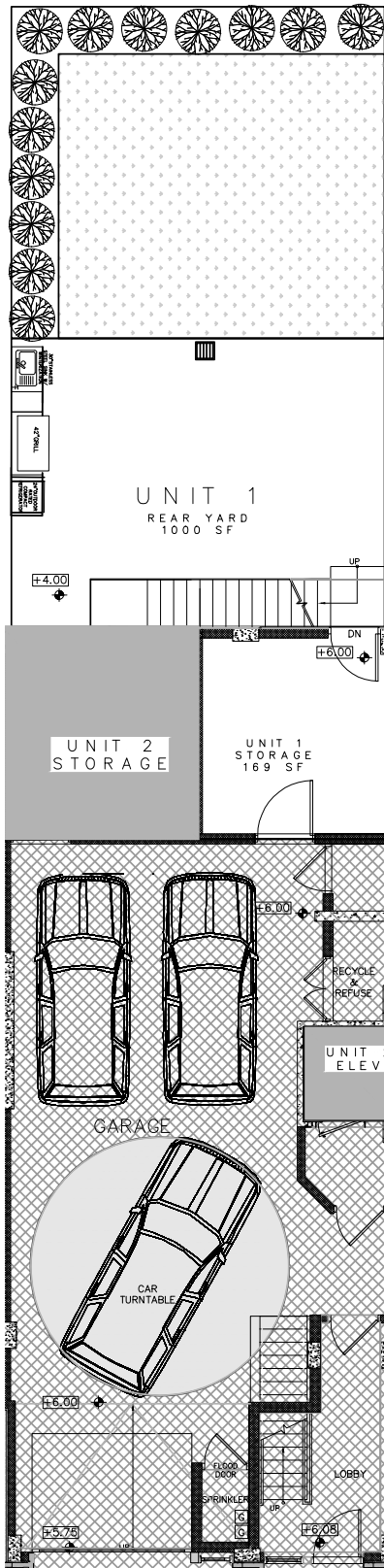
FIRST FLOOR : UNIT 1 SCALE: 3/32"=1'-0"
